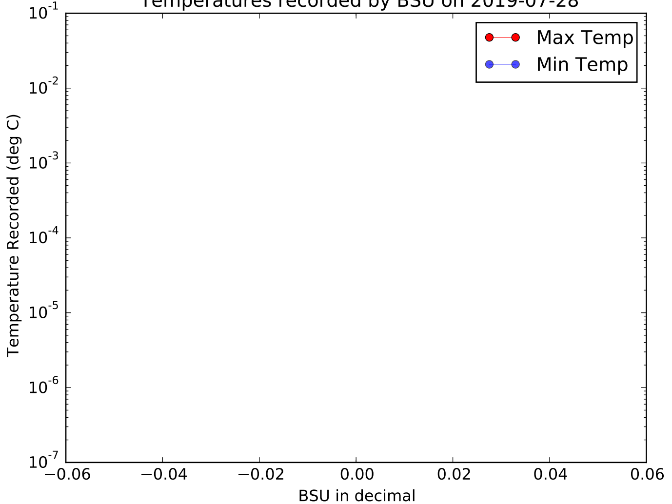
Temperatures recorded by BSU on 2019-07-28
