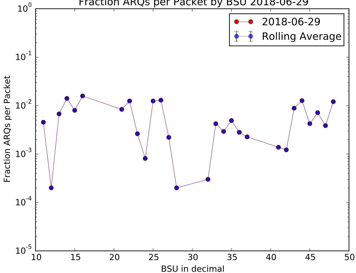
Fraction ARQs per Packet by BSU 2018-06-29
