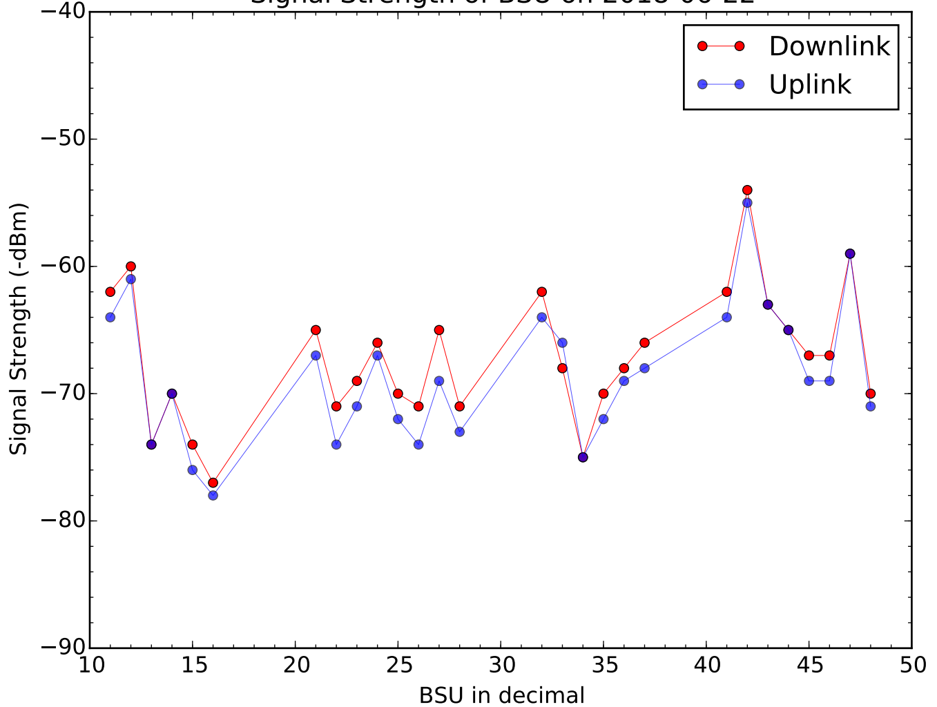
Signal Strength of BSU on 2018-06-22
