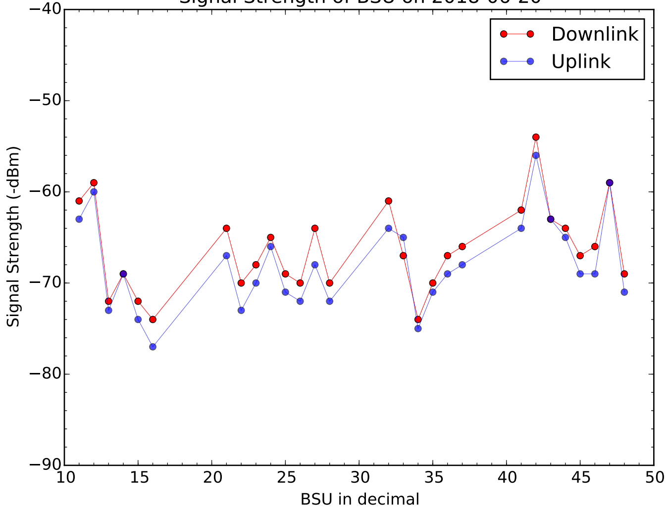
Signal Strength of BSU on 2018-06-20
