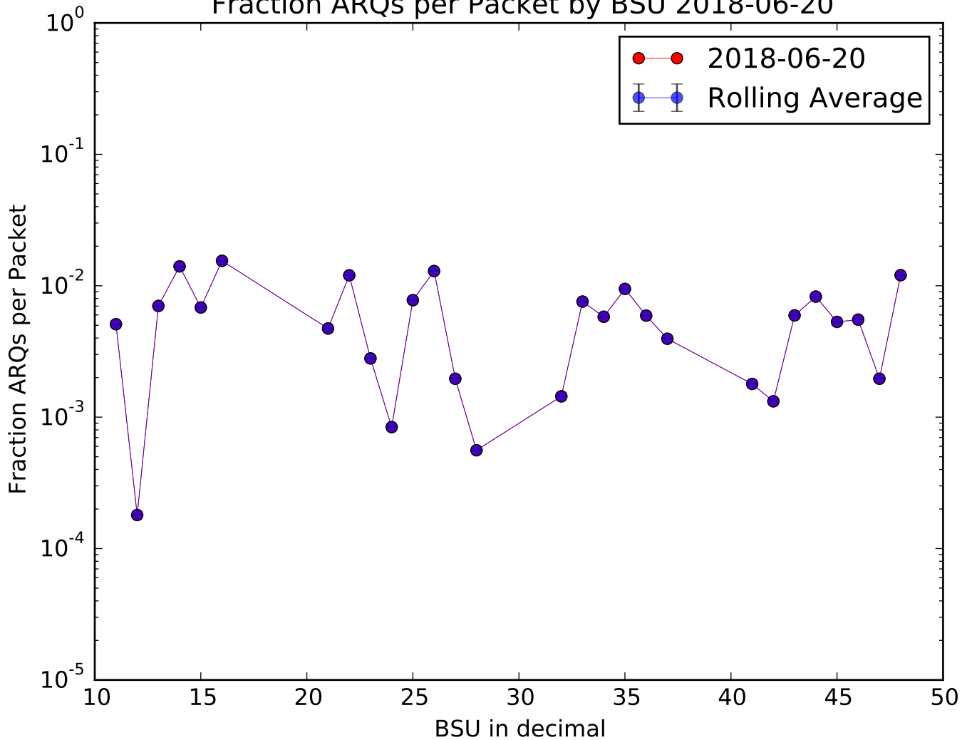
Fraction ARQs per Packet by BSU 2018-06-20
