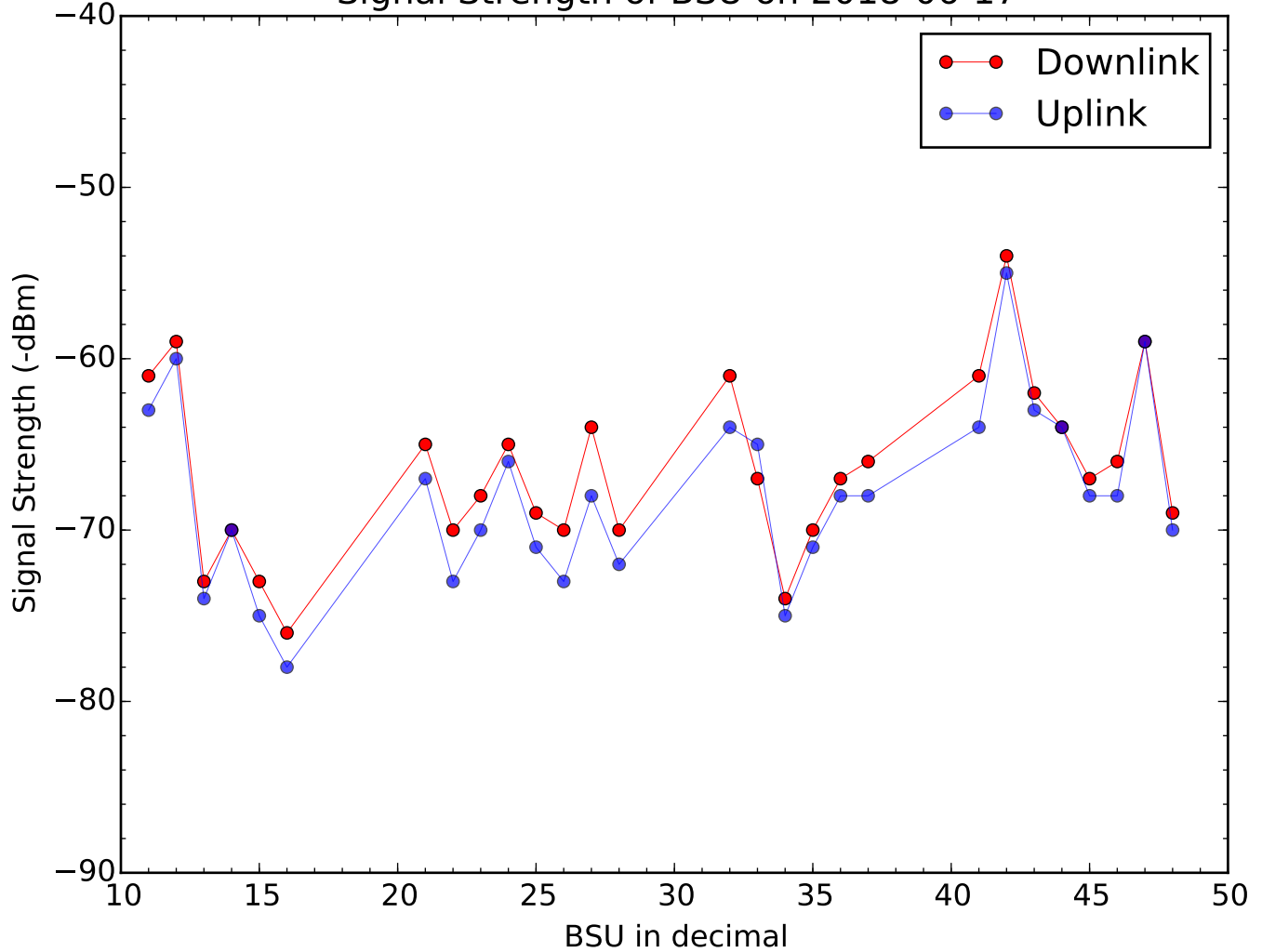
Signal Strength of BSU on 2018-06-17
