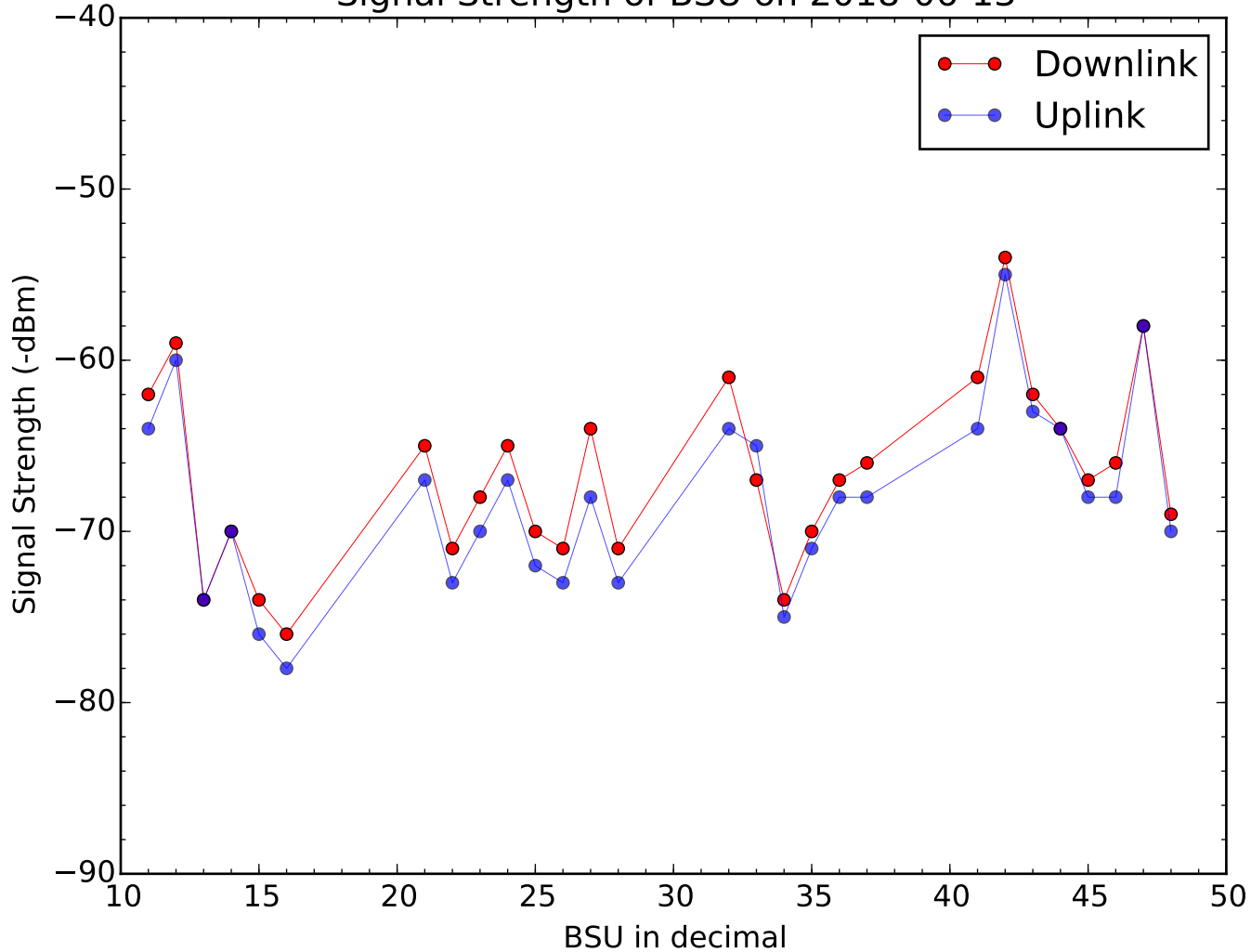
Signal Strength of BSU on 2018-06-13
