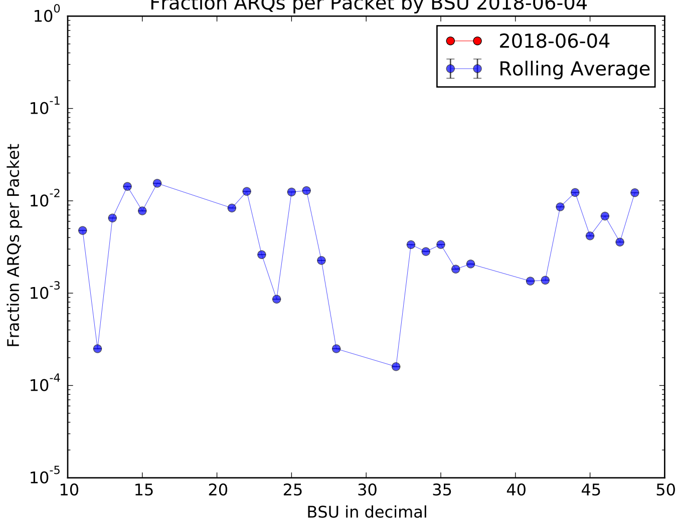
Fraction ARQs per Packet by BSU 2018-06-04
