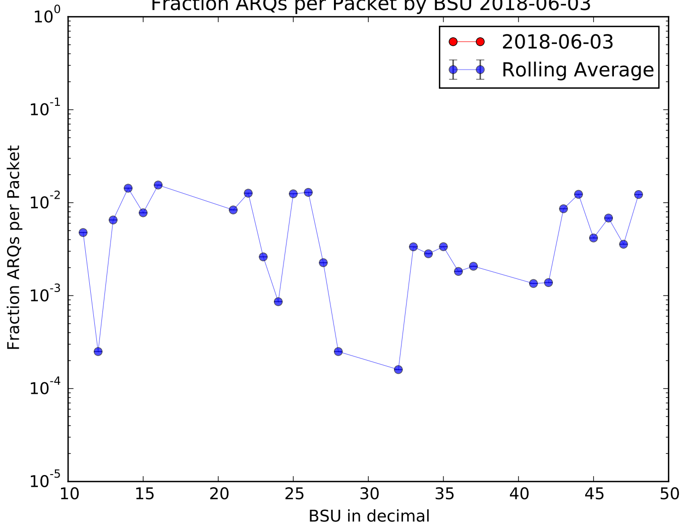
Fraction ARQs per Packet by BSU 2018-06-03
