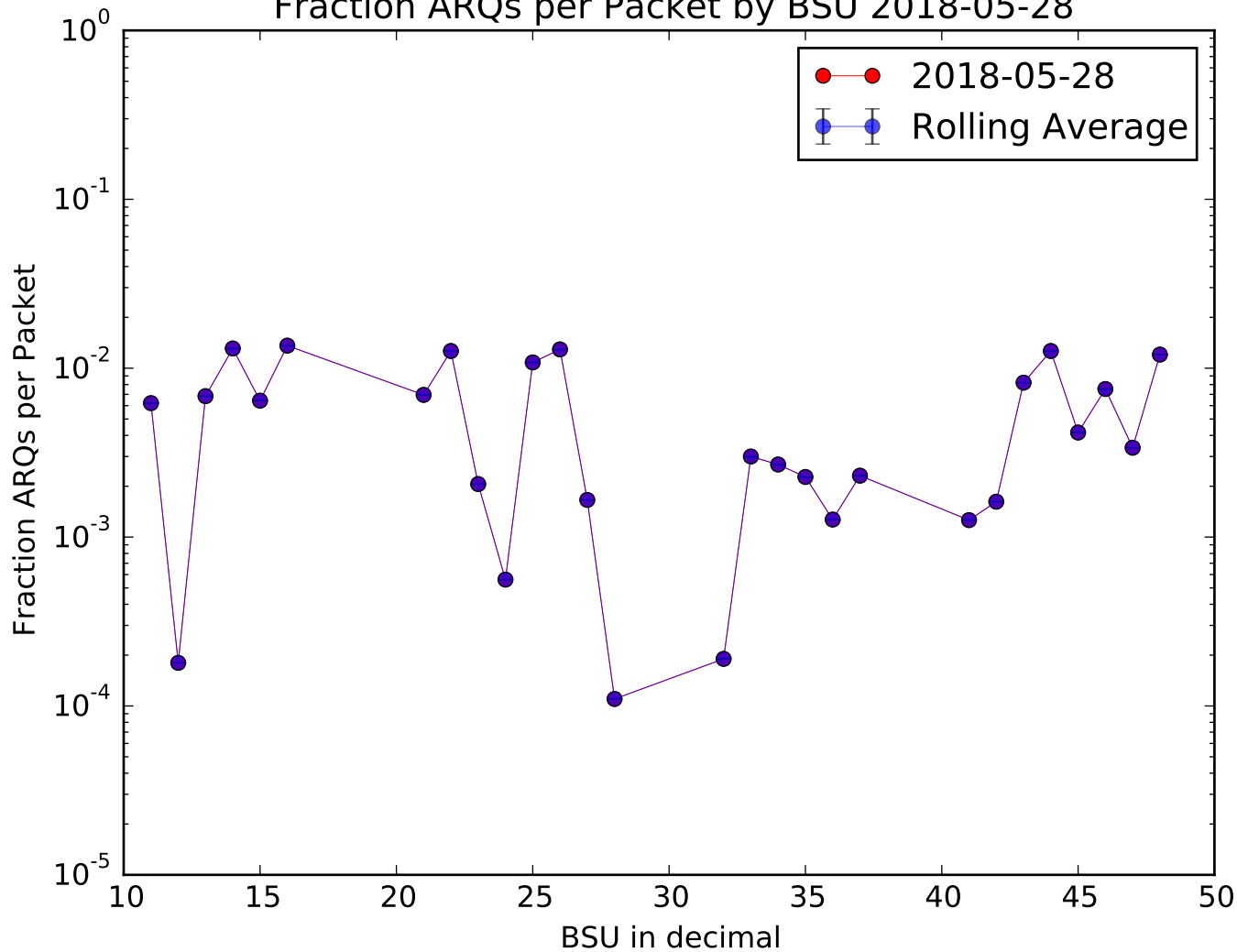
Fraction ARQs per Packet by BSU 2018-05-28
