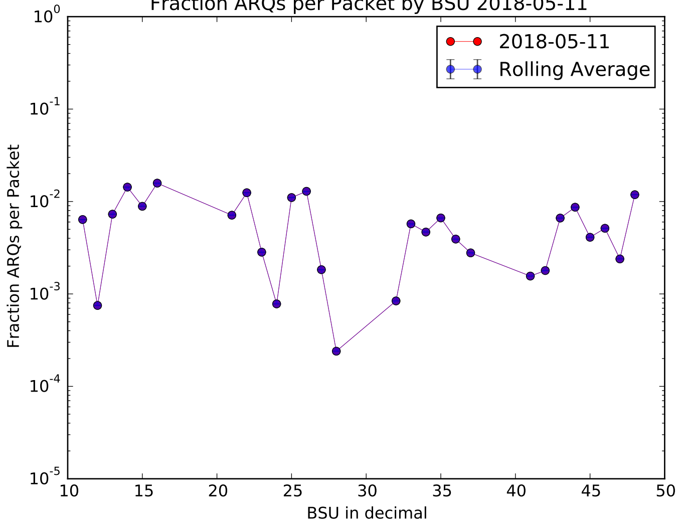
Fraction ARQs per Packet by BSU 2018-05-11
