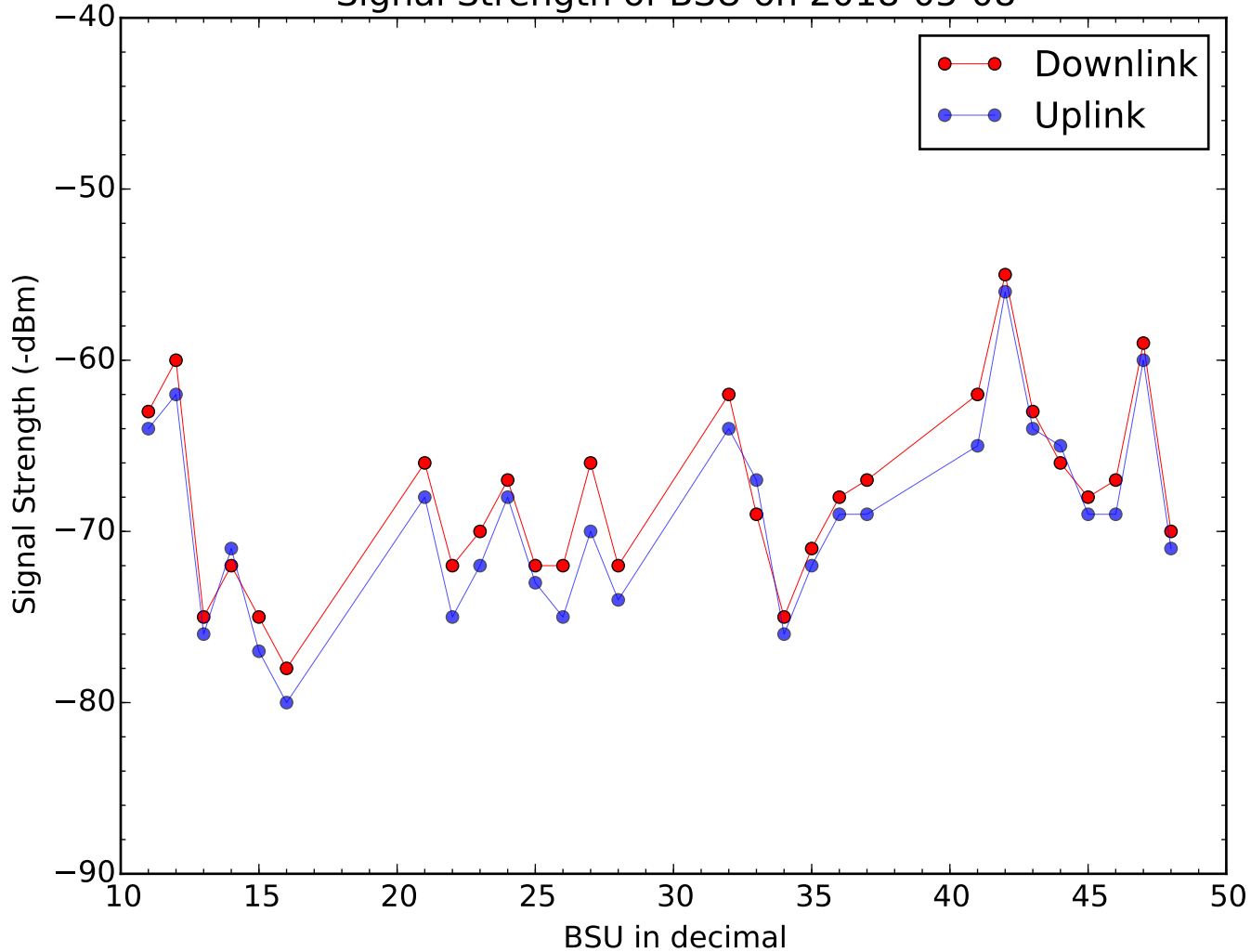
Signal Strength of BSU on 2018-05-08
