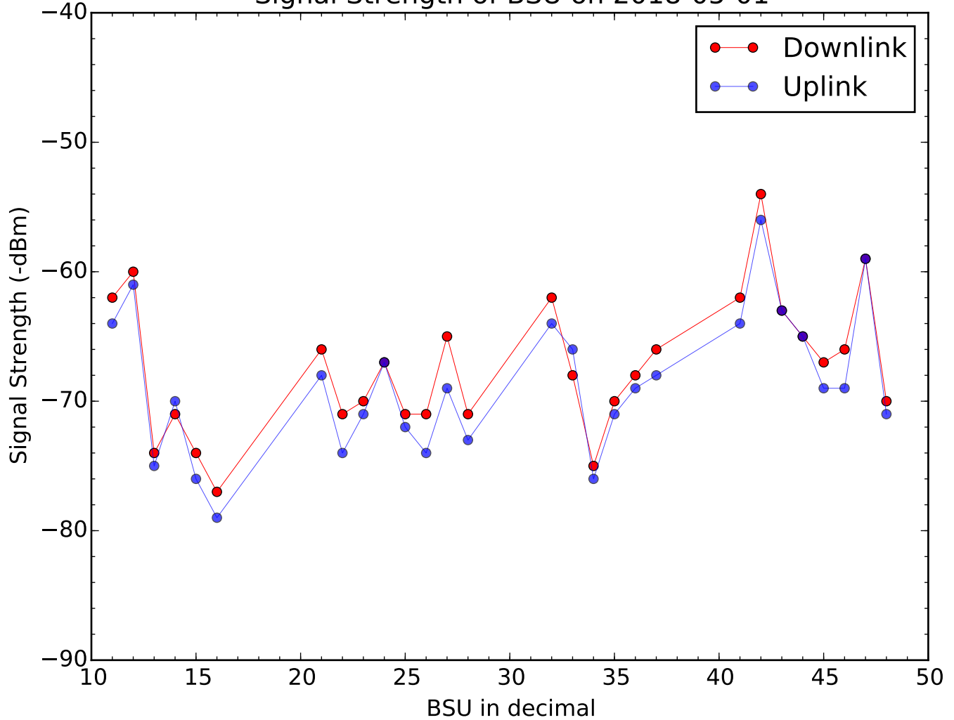
Signal Strength of BSU on 2018-05-01
