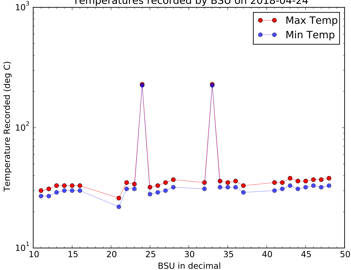
Temperatures recorded by BSU on 2018-04-24
