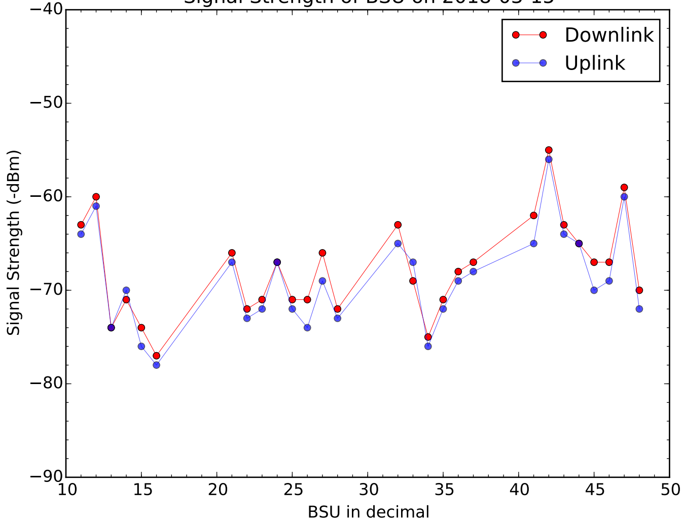
Signal Strength of BSU on 2018-03-15
