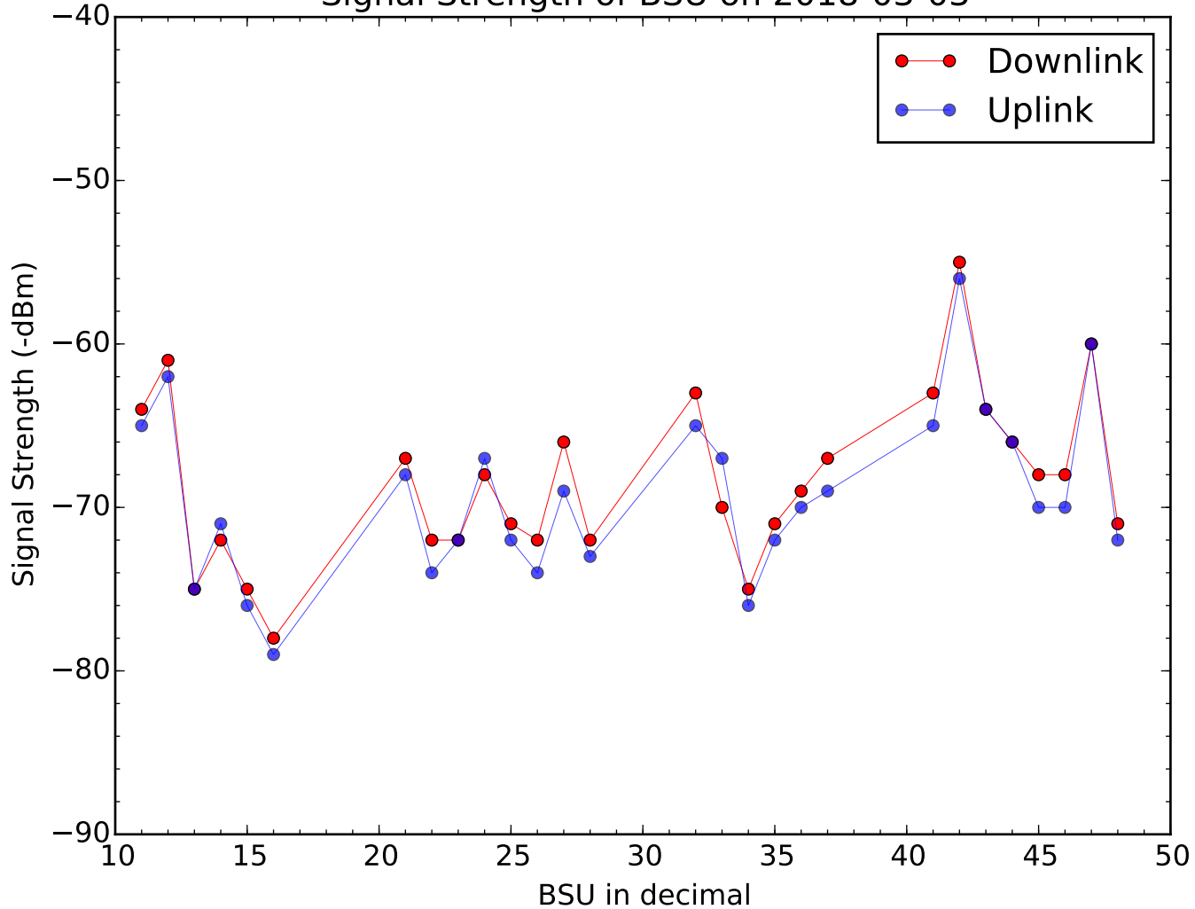
Signal Strength of BSU on 2018-03-03
