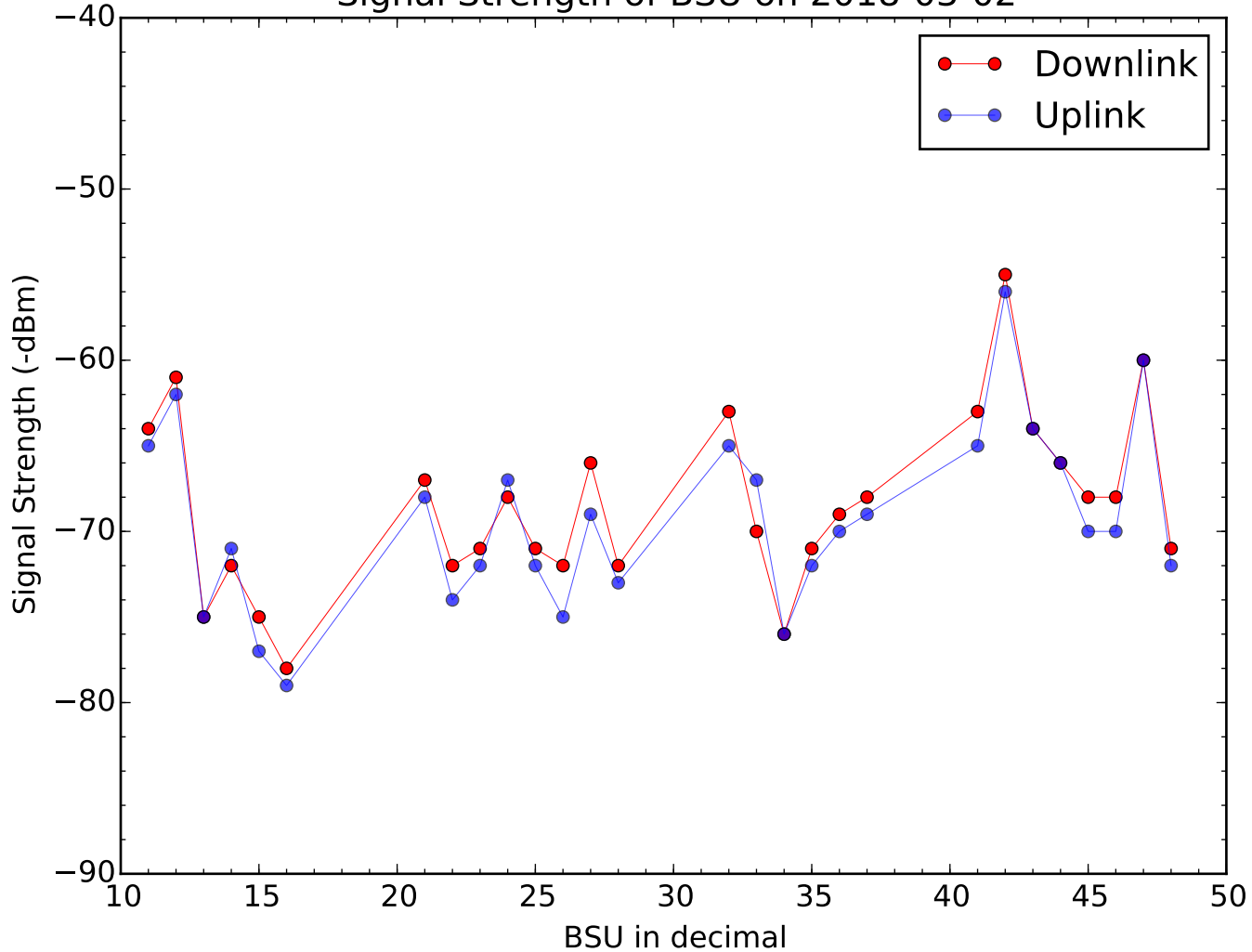
Signal Strength of BSU on 2018-03-02
