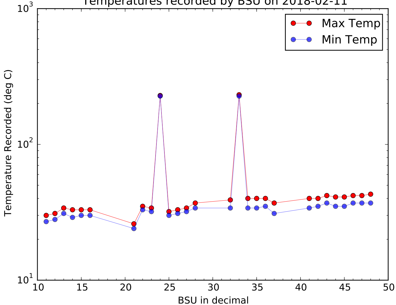
Temperatures recorded by BSU on 2018-02-11
