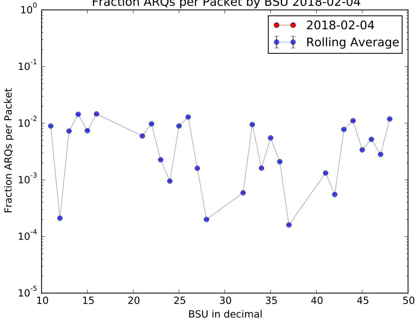
Fraction ARQs per Packet by BSU 2018-02-04
