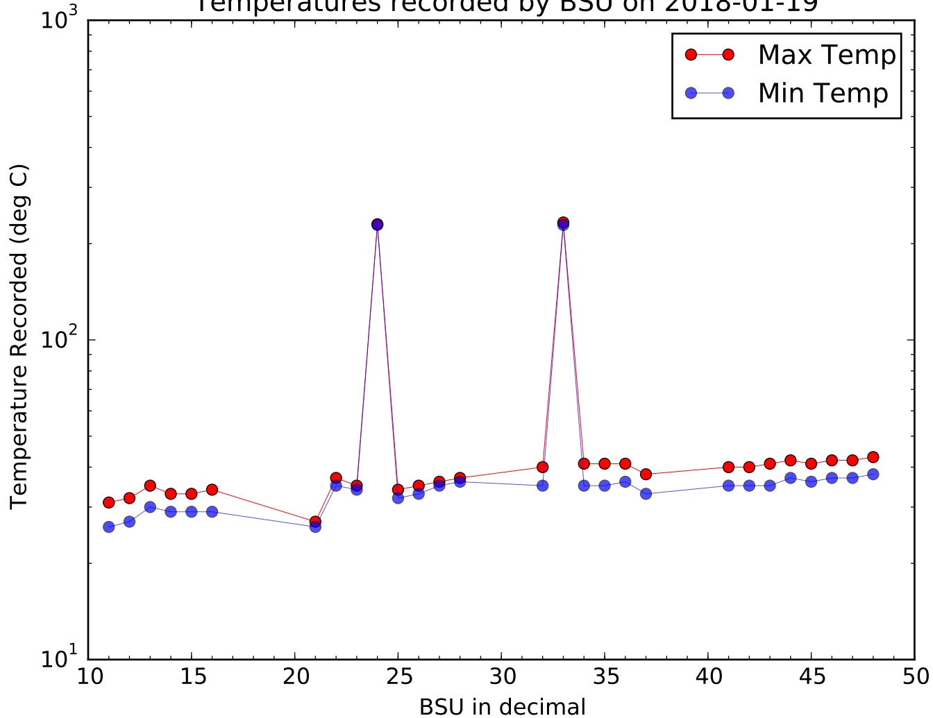
Temperatures recorded by BSU on 2018-01-19
