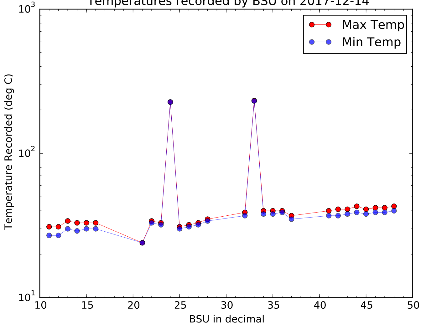
Temperatures recorded by BSU on 2017-12-14
