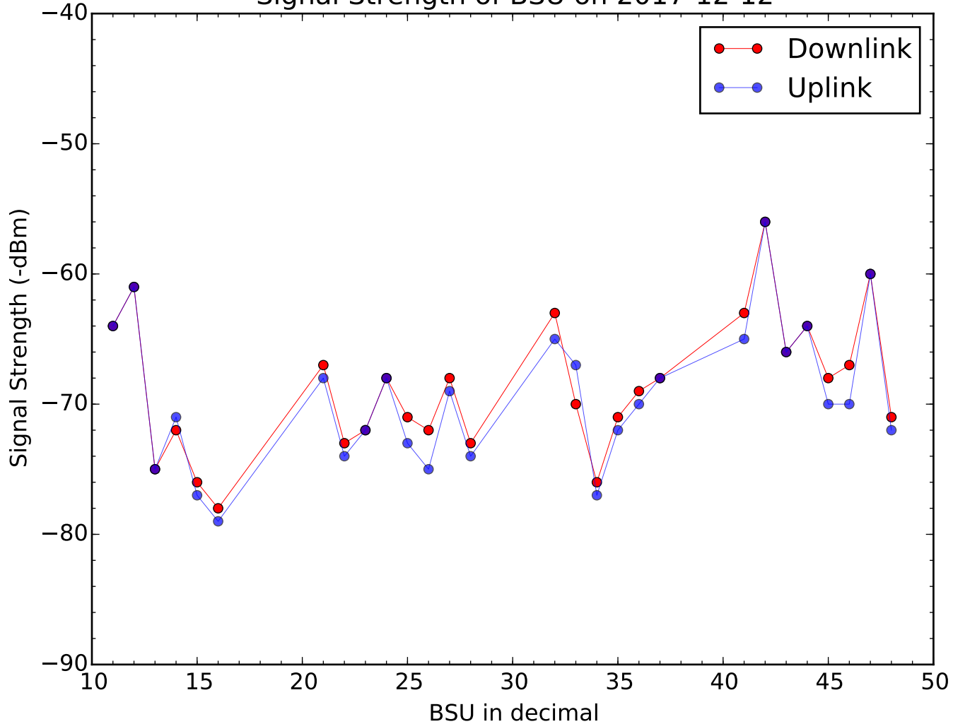
Signal Strength of BSU on 2017-12-12
