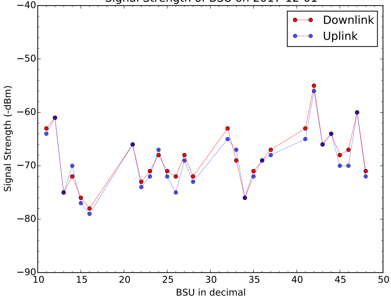
Signal Strength of BSU on 2017-12-01
