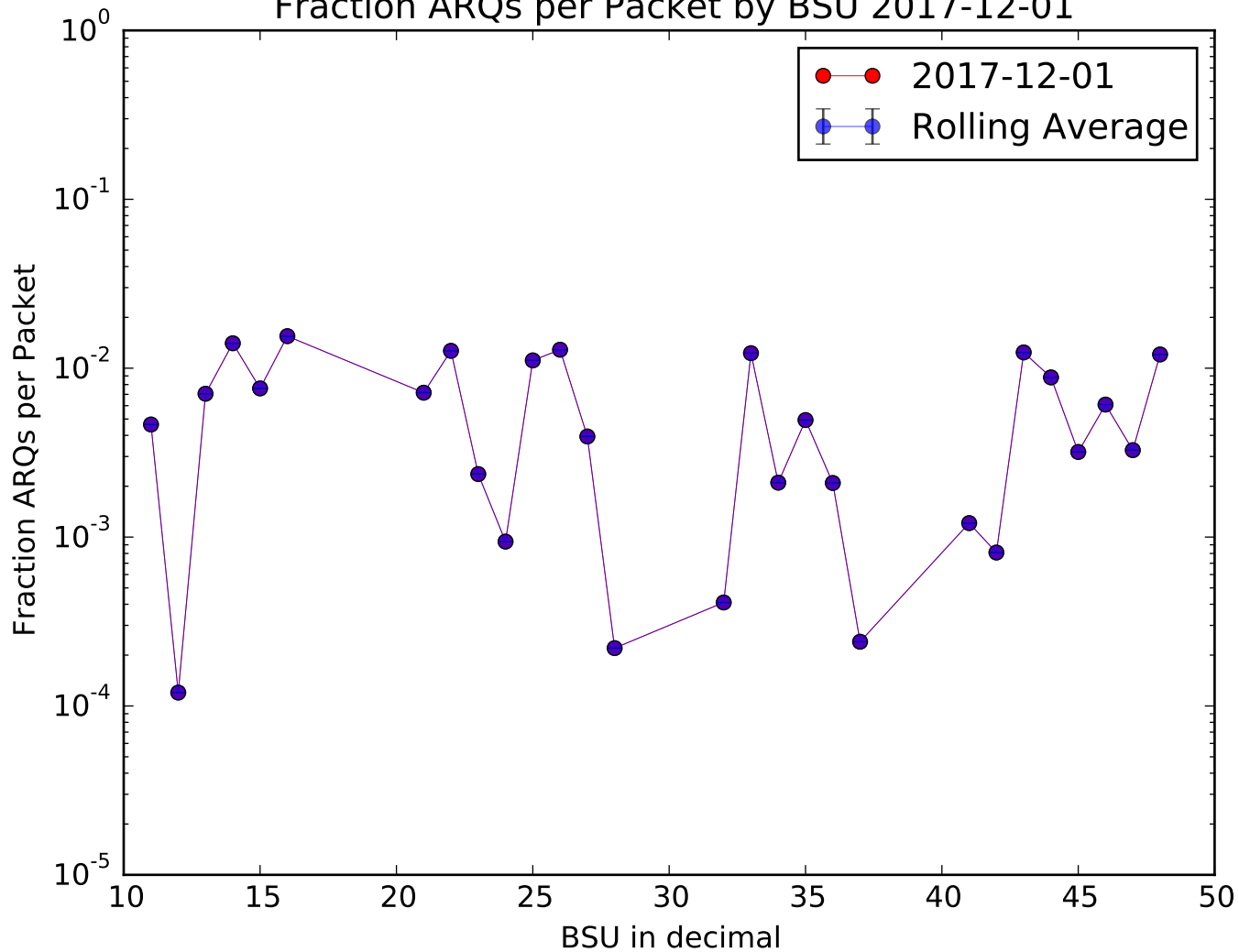
Fraction ARQs per Packet by BSU 2017-12-01
