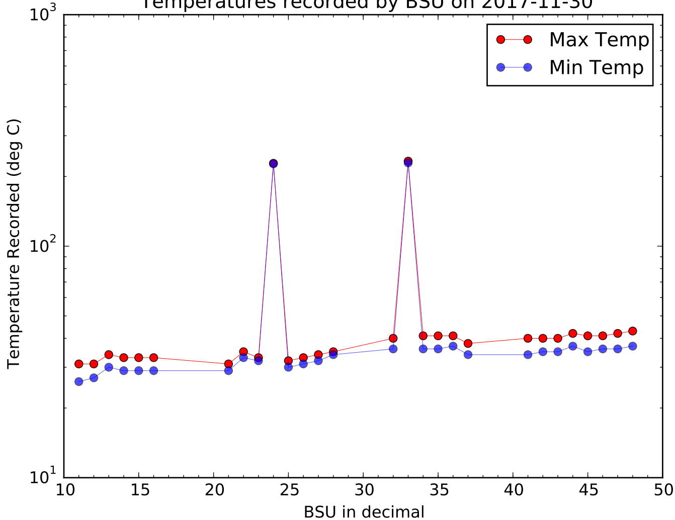
Temperatures recorded by BSU on 2017-11-30
