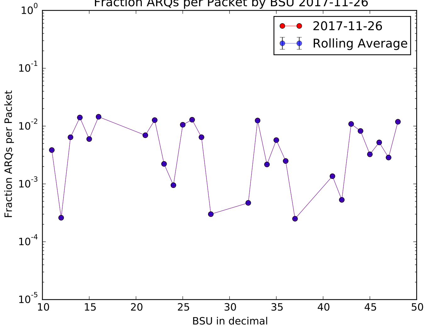
Fraction ARQs per Packet by BSU 2017-11-26
