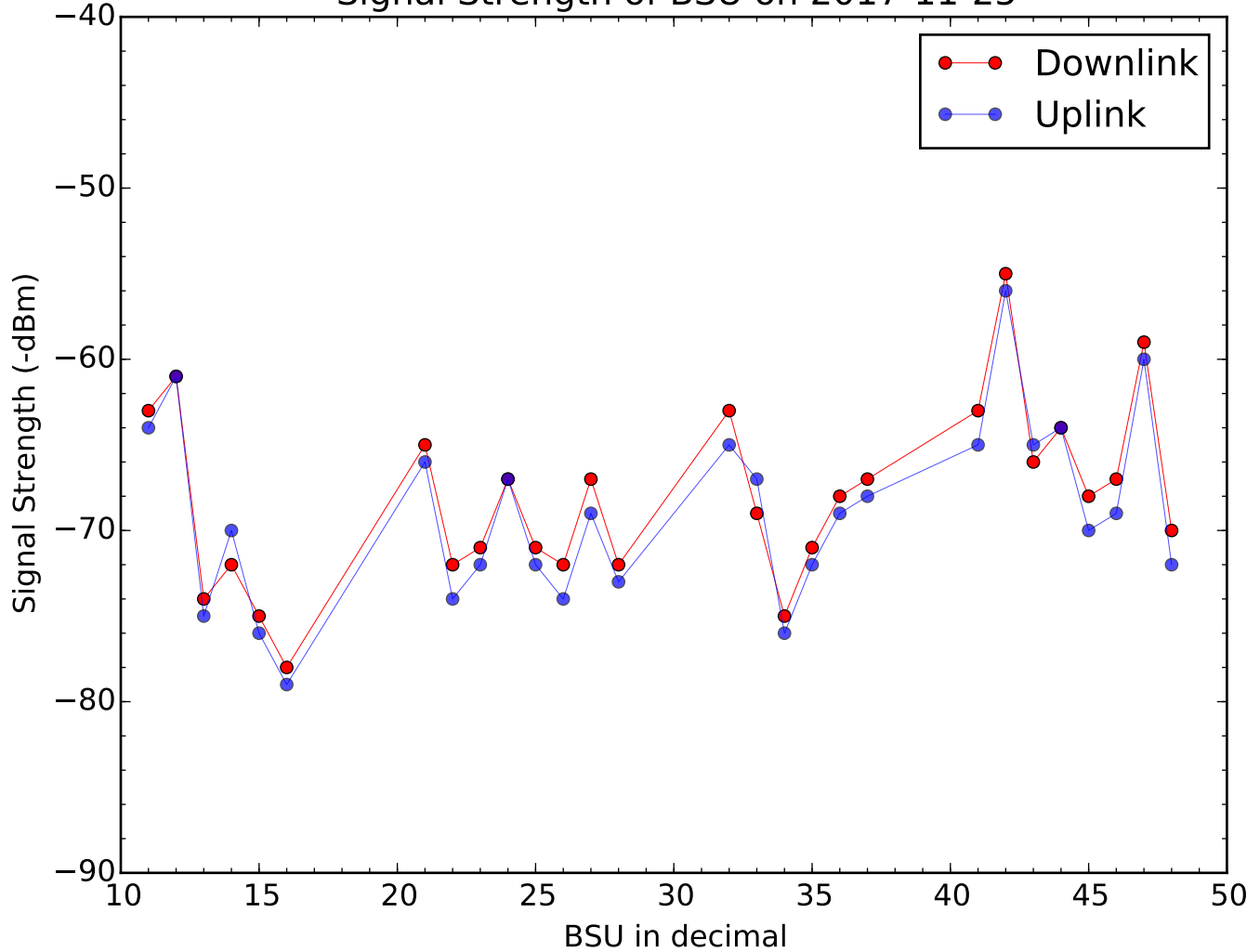
Signal Strength of BSU on 2017-11-25
