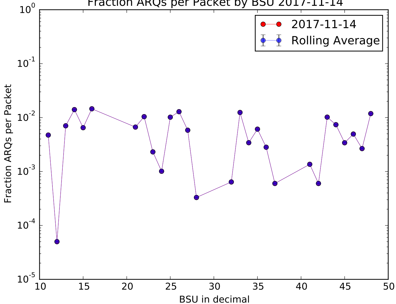
Fraction ARQs per Packet by BSU 2017-11-14
