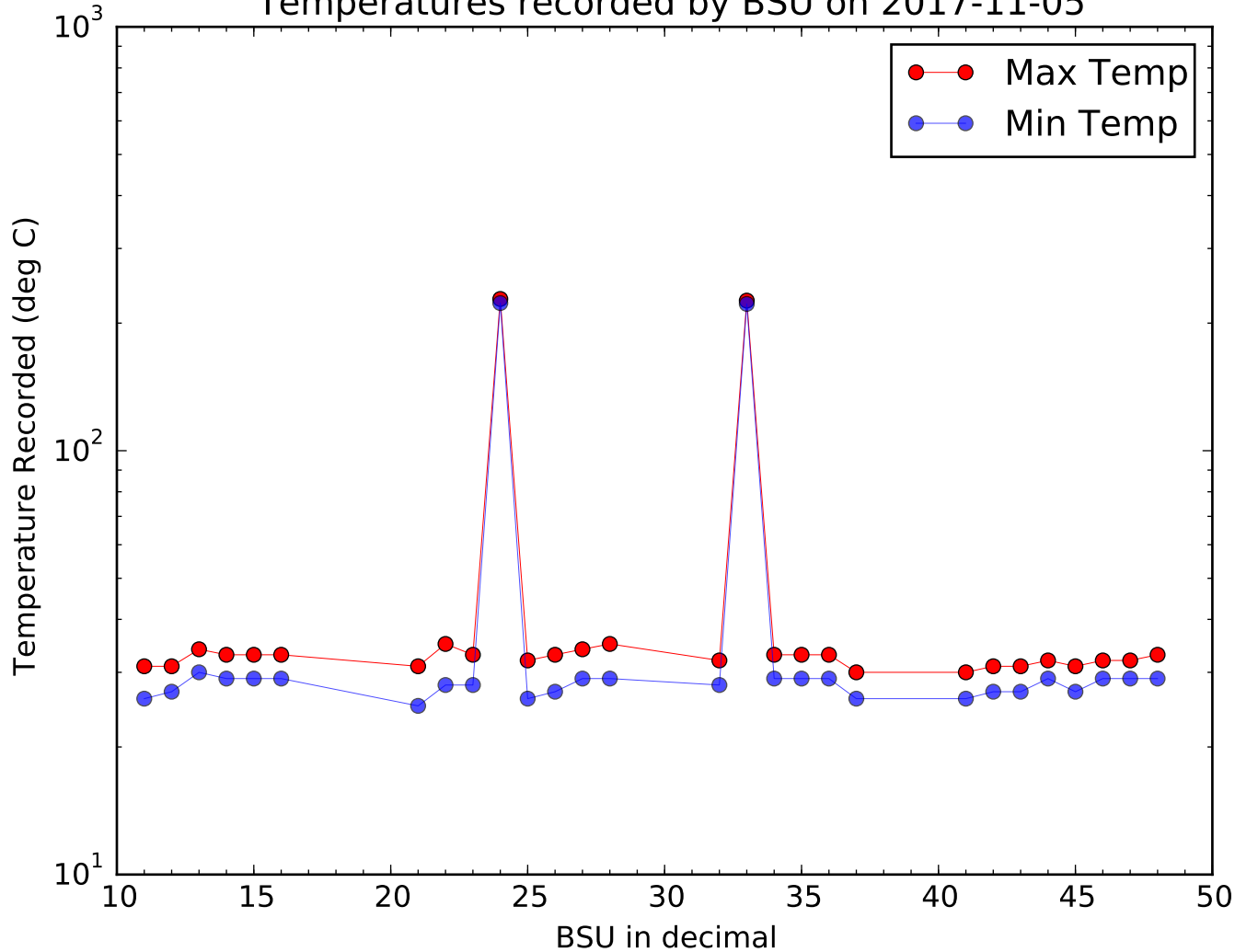
Temperatures recorded by BSU on 2017-11-05
