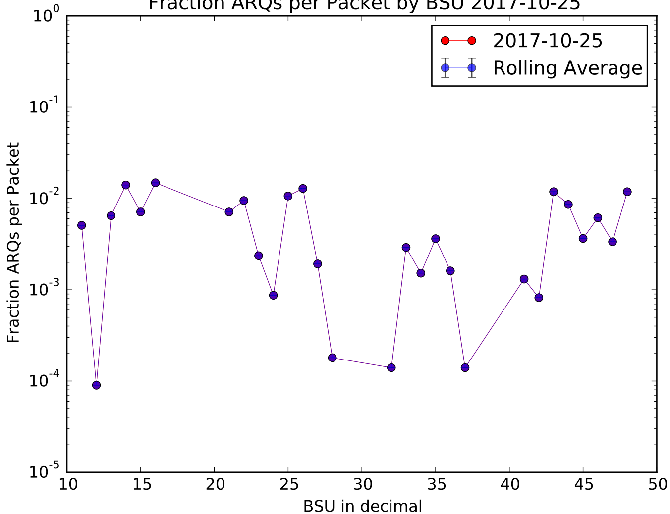
Fraction ARQs per Packet by BSU 2017-10-25
