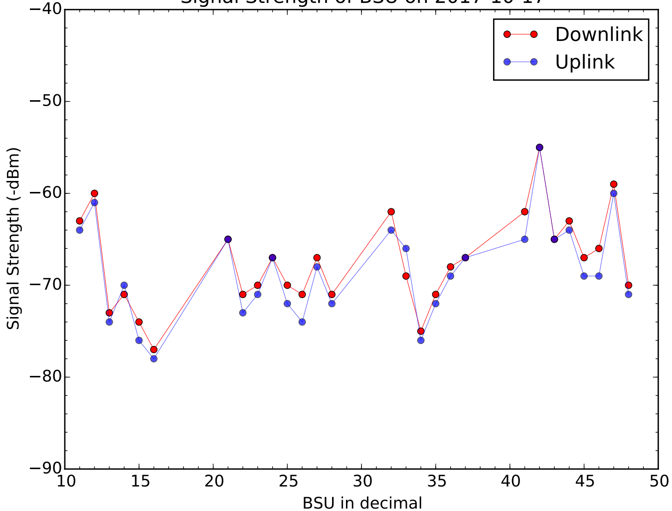
Signal Strength of BSU on 2017-10-17
