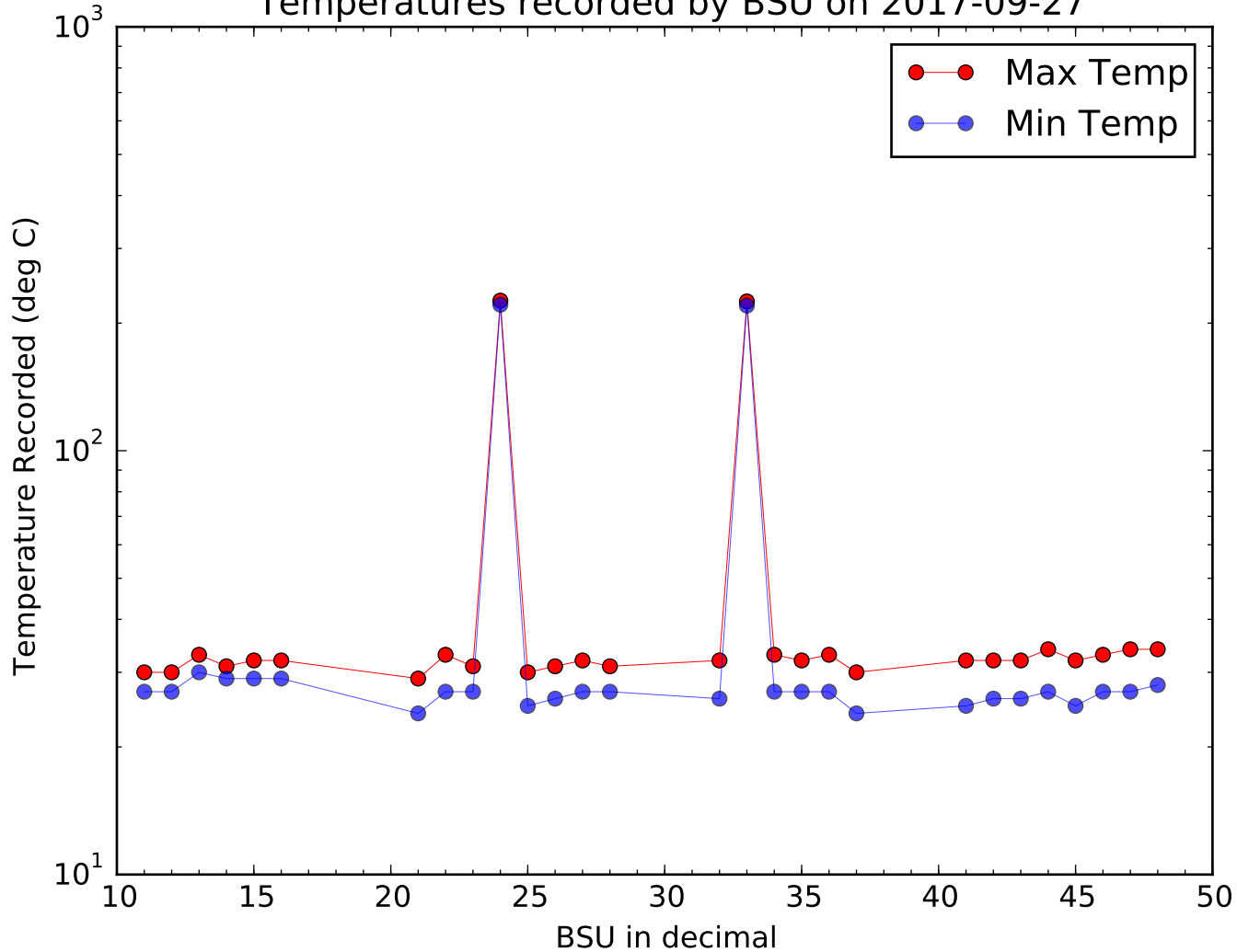
Temperatures recorded by BSU on 2017-09-27
