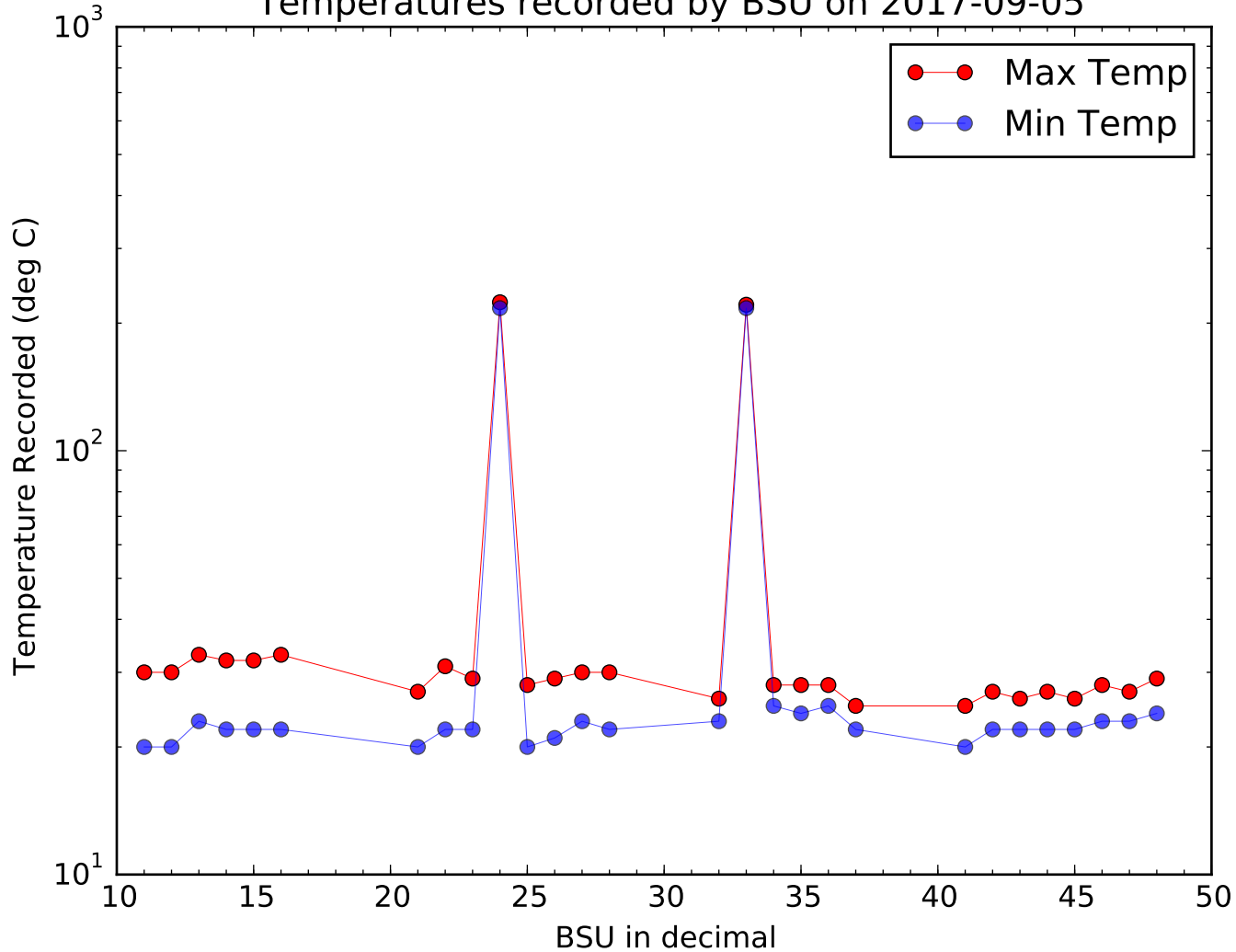
Temperatures recorded by BSU on 2017-09-05
