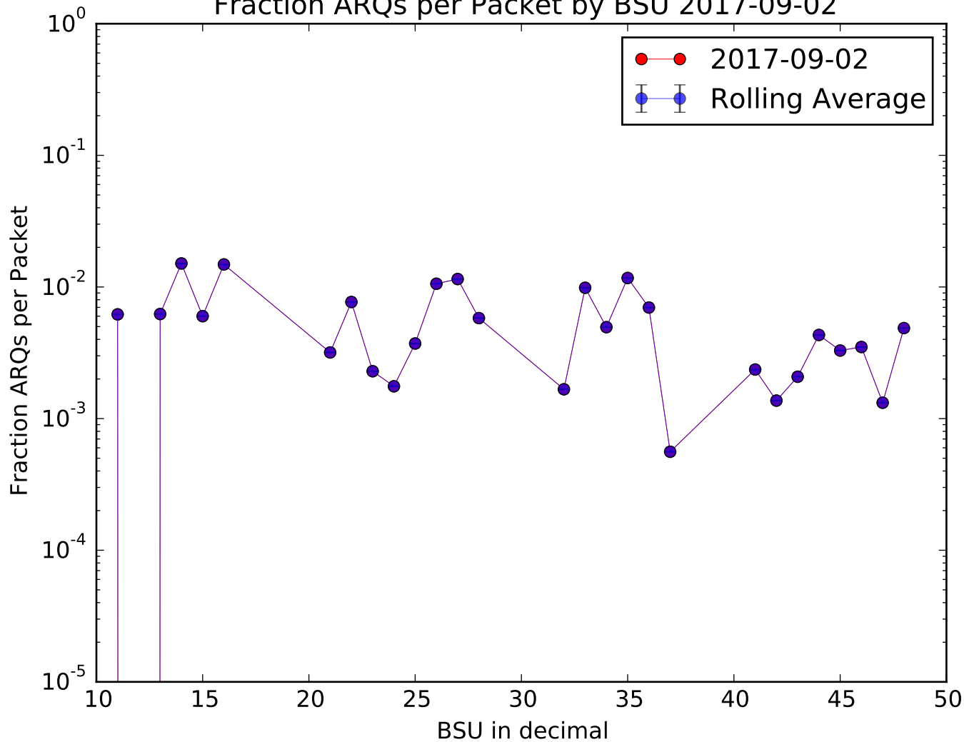
Fraction ARQs per Packet by BSU 2017-09-02
