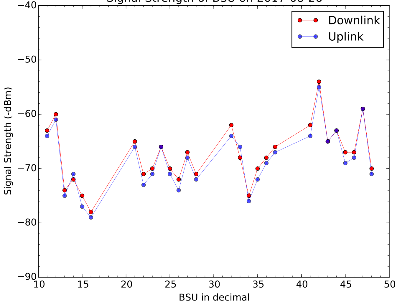
Signal Strength of BSU on 2017-08-26
