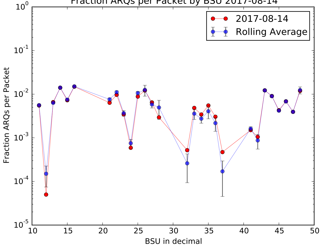
Fraction ARQs per Packet by BSU 2017-08-14
