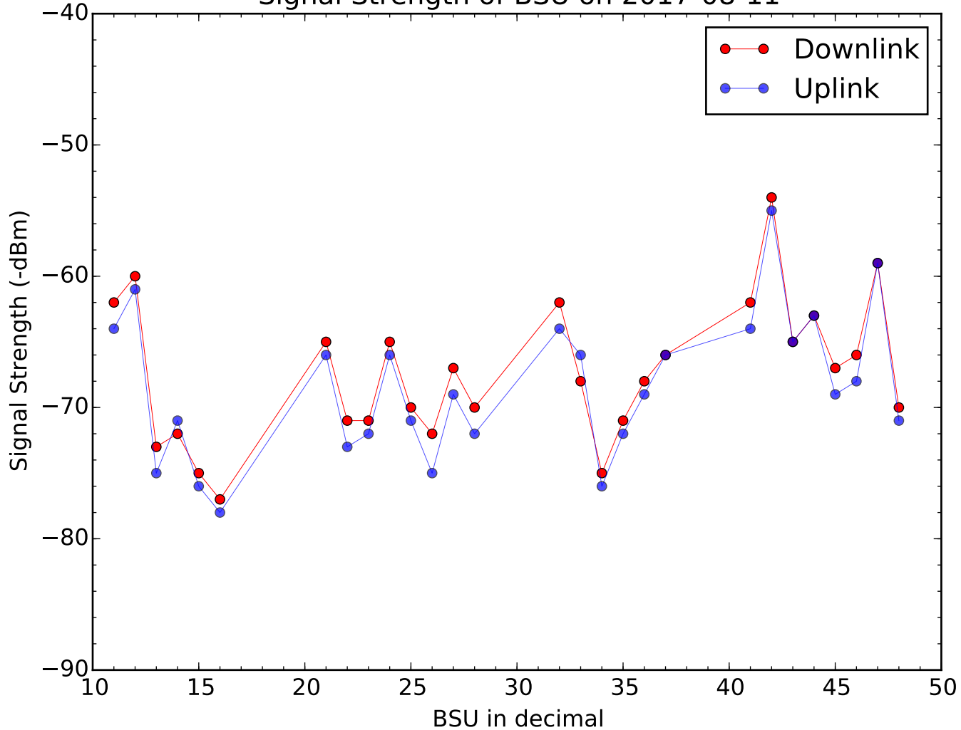
Signal Strength of BSU on 2017-08-11
