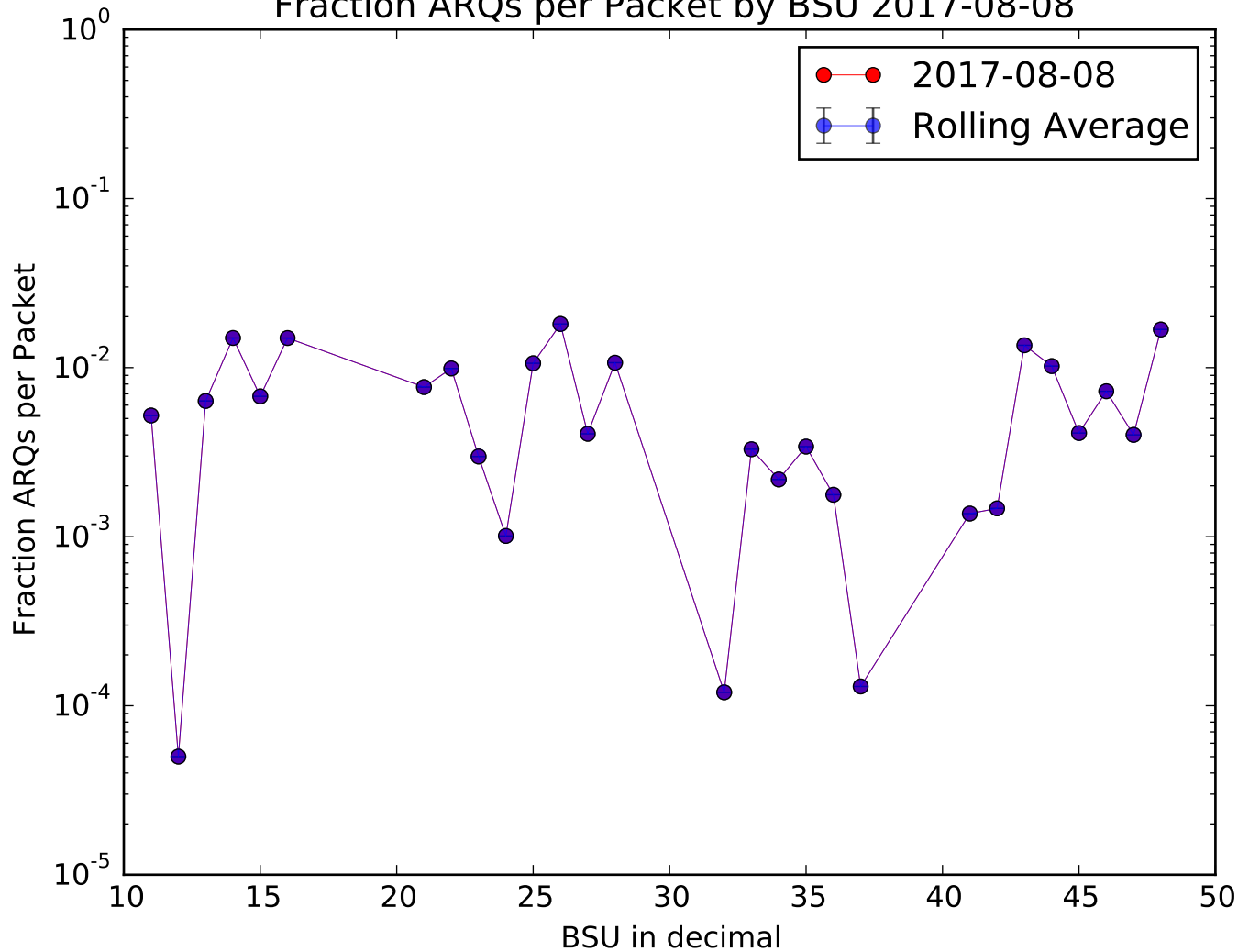
Fraction ARQs per Packet by BSU 2017-08-08
