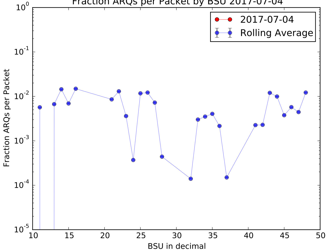
Fraction ARQs per Packet by BSU 2017-07-04
