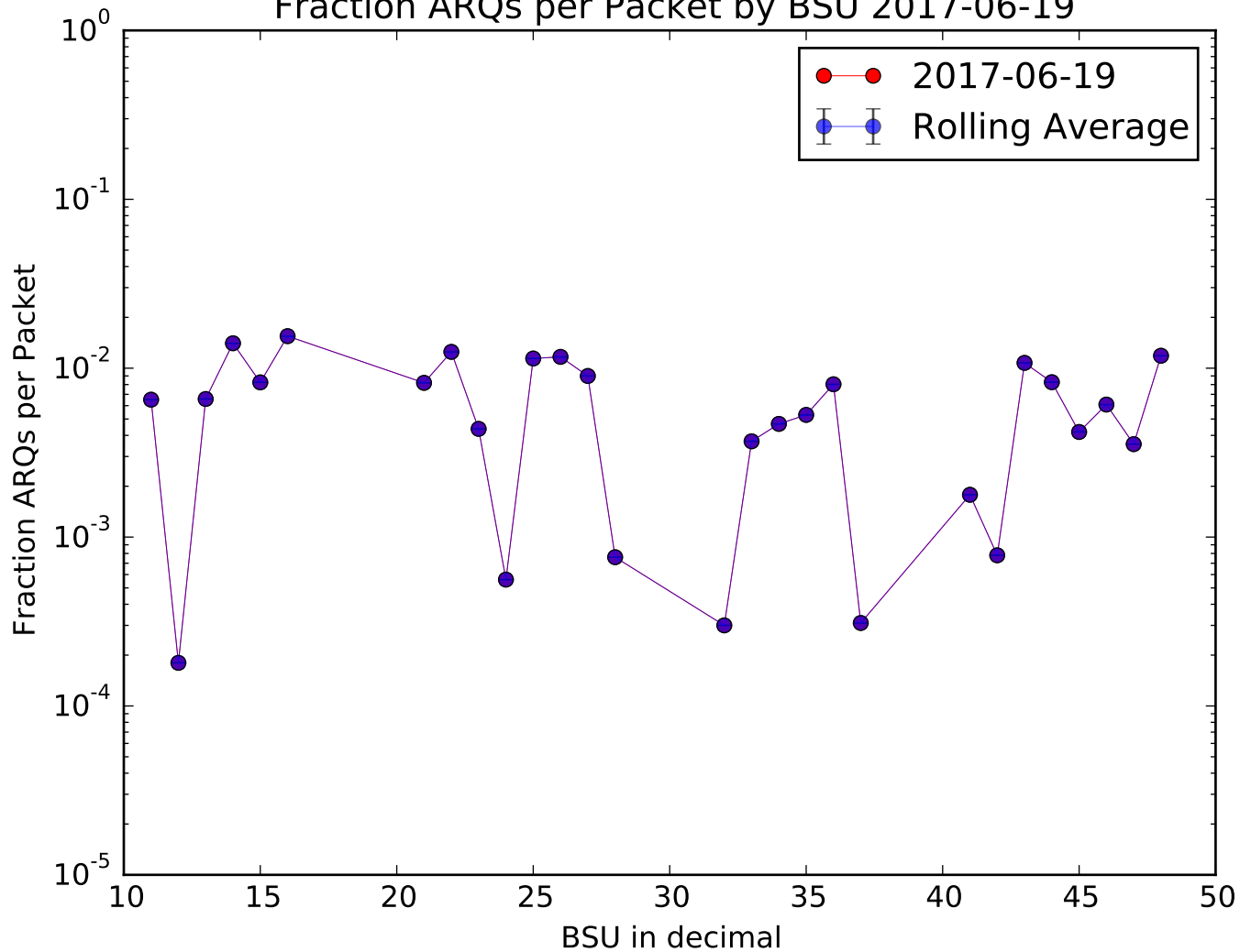
Fraction ARQs per Packet by BSU 2017-06-19
