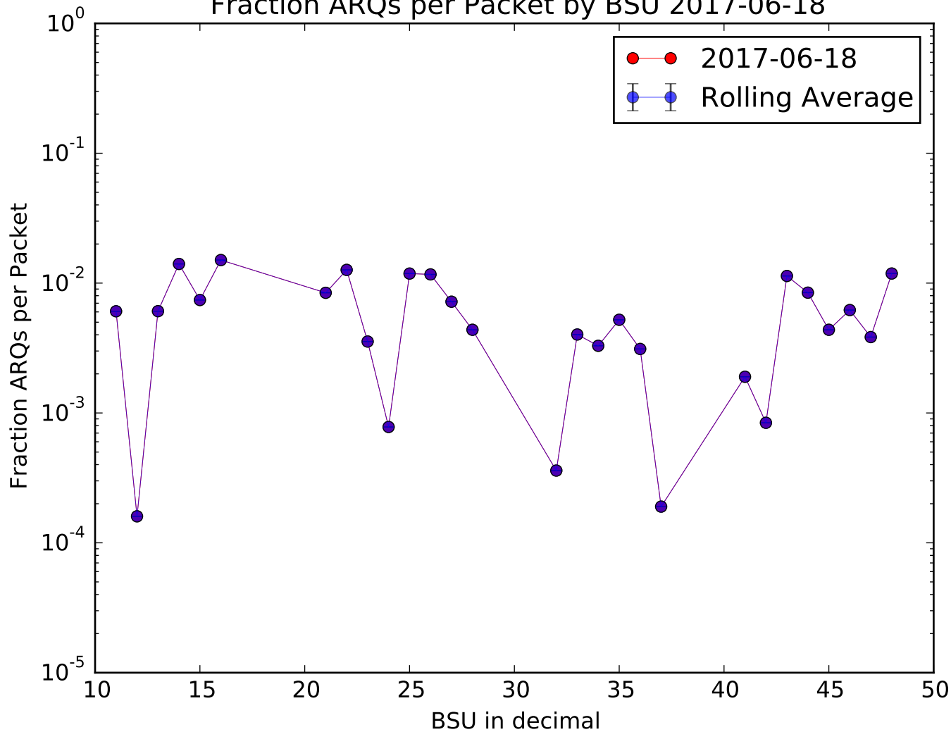
Fraction ARQs per Packet by BSU 2017-06-18
