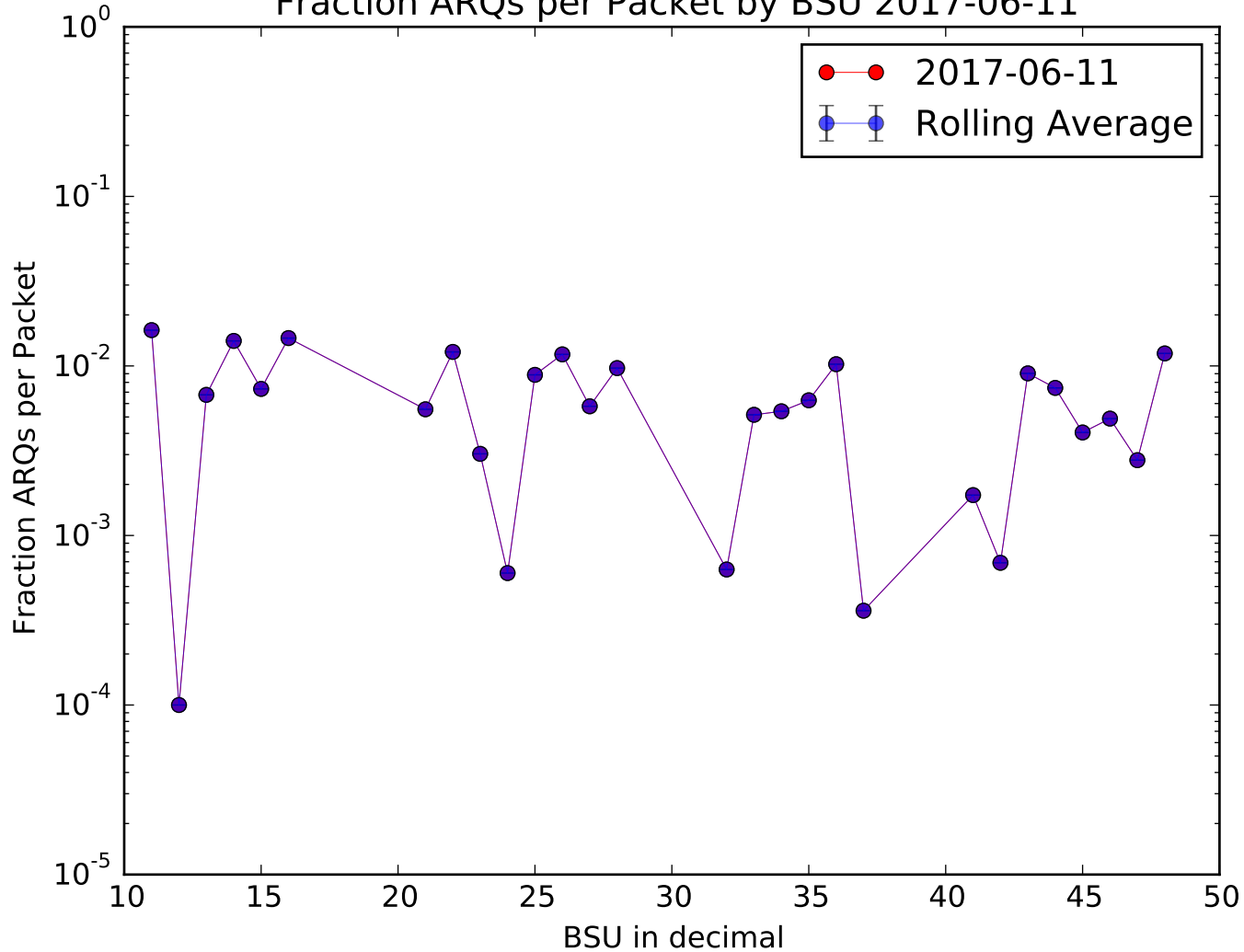
Fraction ARQs per Packet by BSU 2017-06-11
