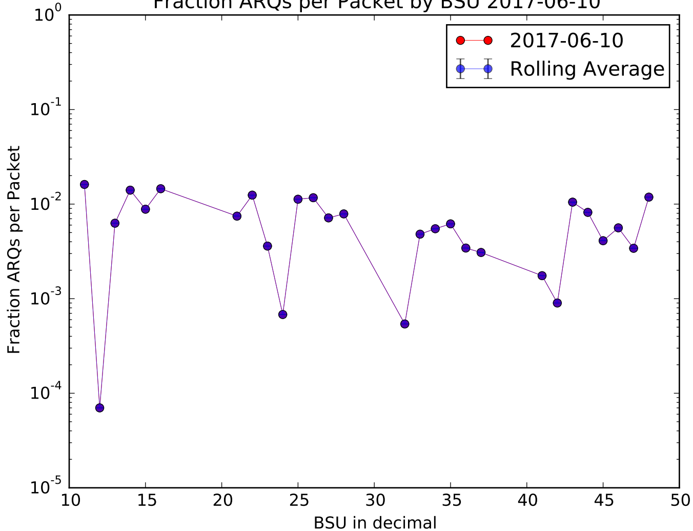
Fraction ARQs per Packet by BSU 2017-06-10
