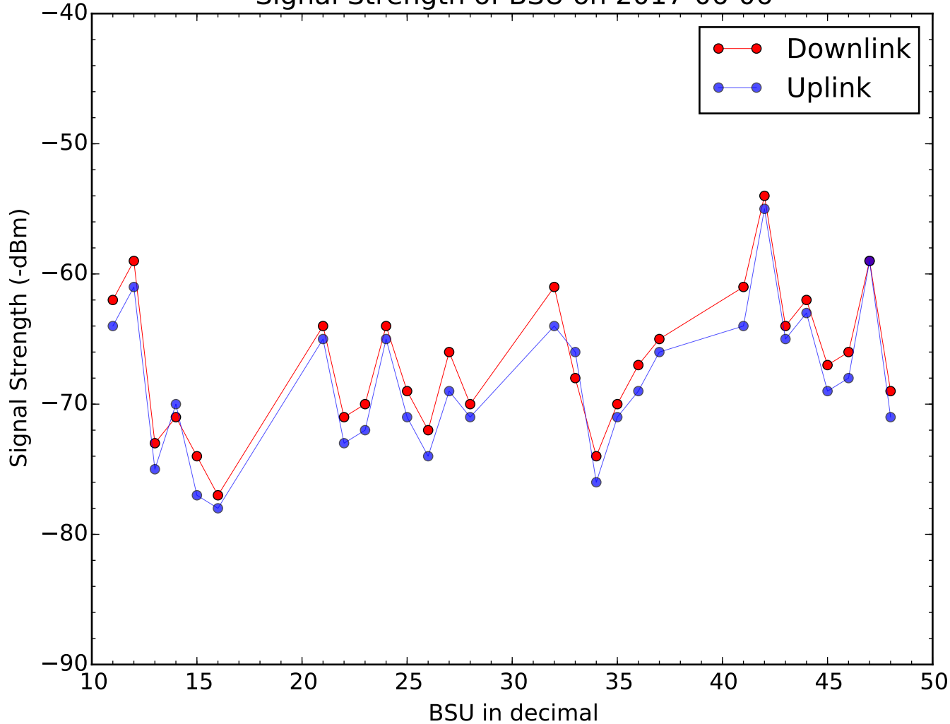
Signal Strength of BSU on 2017-06-06
