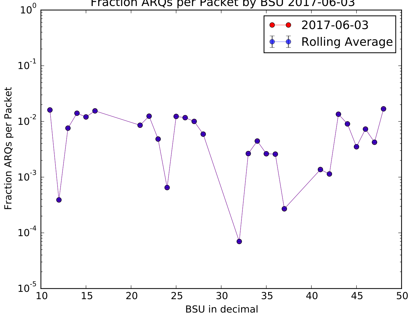
Fraction ARQs per Packet by BSU 2017-06-03
