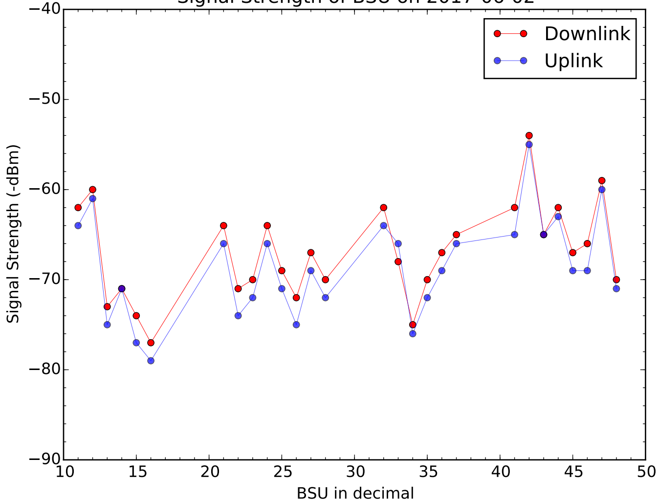
Signal Strength of BSU on 2017-06-02
