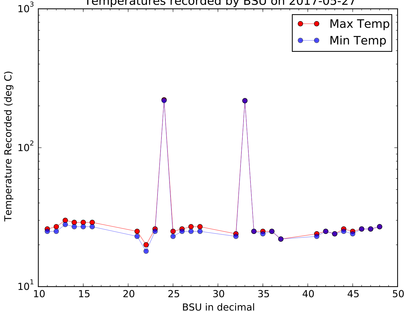
Temperatures recorded by BSU on 2017-05-27
