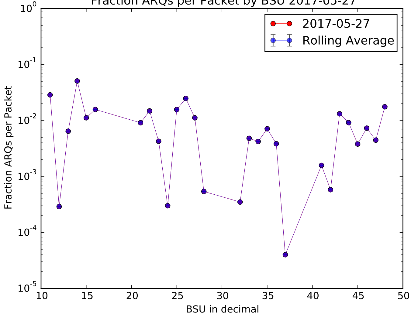
Fraction ARQs per Packet by BSU 2017-05-27
