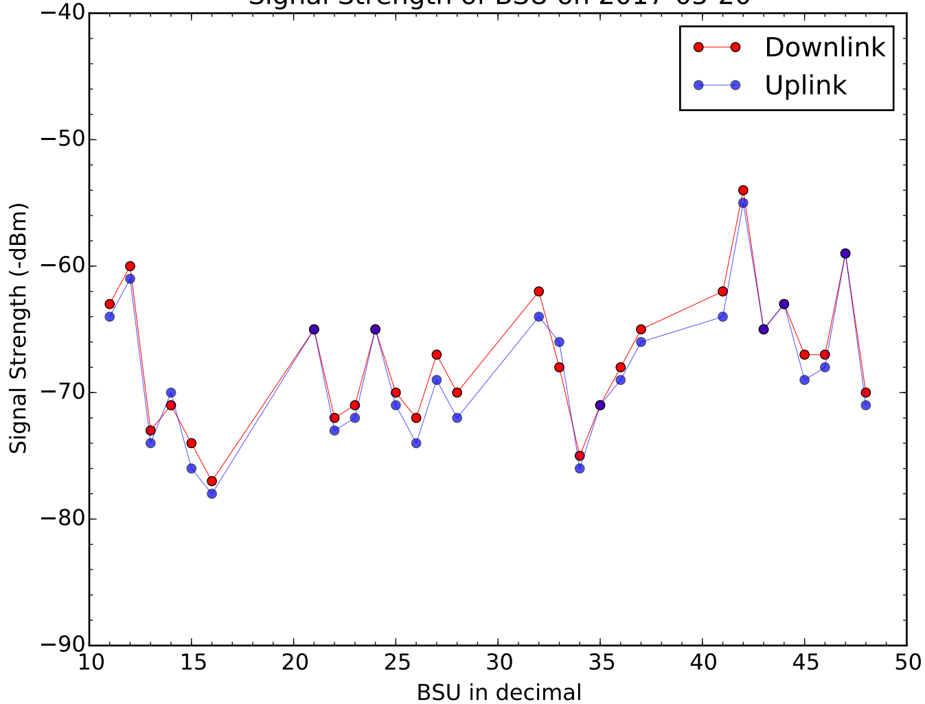
Signal Strength of BSU on 2017-05-20
