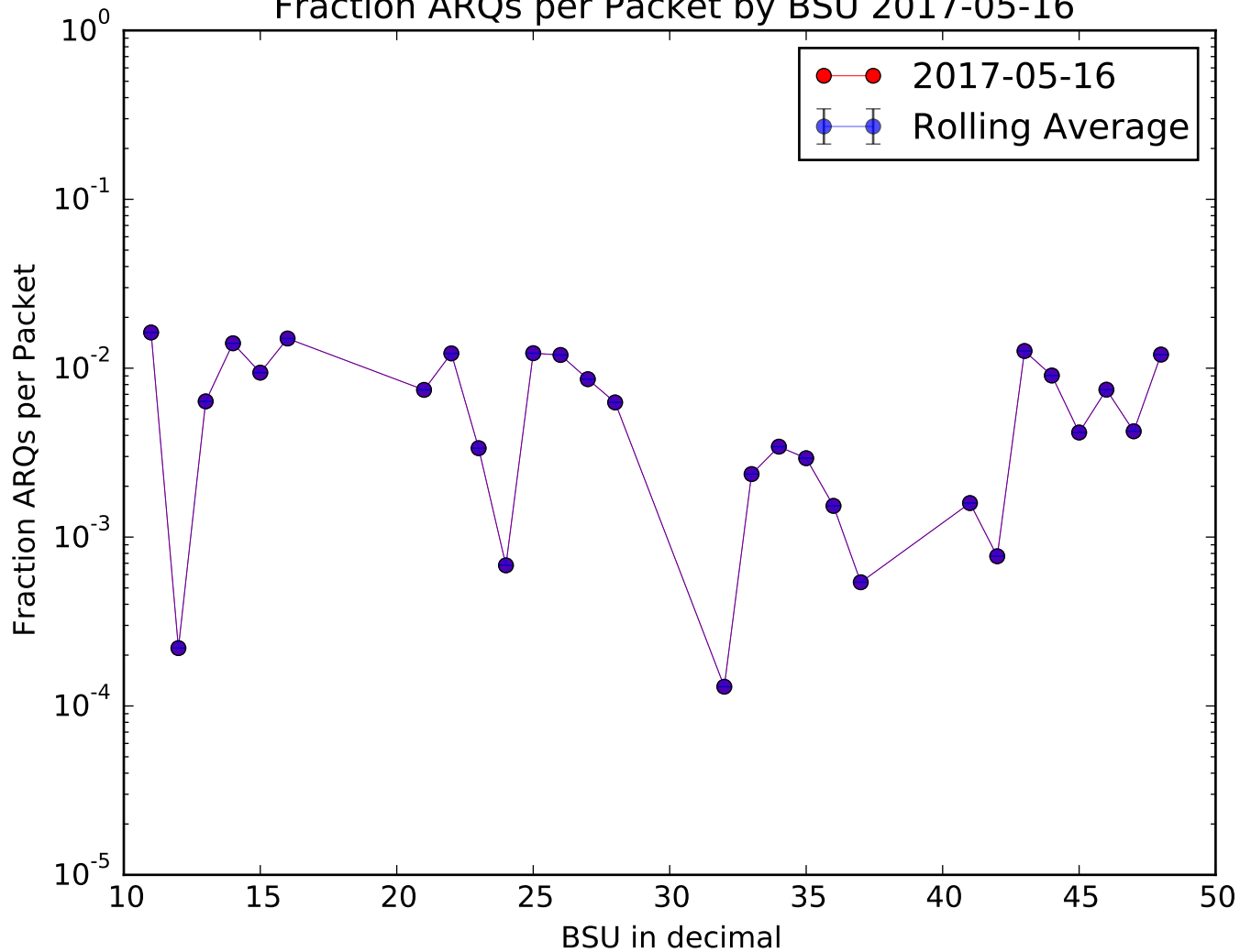
Fraction ARQs per Packet by BSU 2017-05-16
